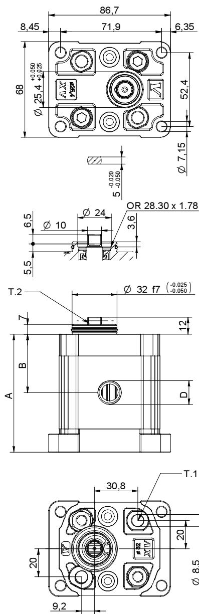
TIPO Peso A B D D kg mm mm IN OUT X1T/0.9 0,950 73,5 36,3 3/8" BSPP 3/8" BSPP X1T/1.2 0,970 74,5 36,8 3/8" BSPP 3/8" BSPP X1T/1.7 1,010 76,0 37,5 3/8" BSPP 3/8" BSPP X1T/2.2 1,030 78,0 38,5 3/8" BSPP 3/8" BSPP X1T/2.6 1,060 80,0 39,5 3/8" BSPP 3/8" BSPP X1T/3.2 1,090 82,0 40,5 3/8" BSPP 3/8" BSPP X1T/3.8 1,120 84,0 41,5 3/8" BSPP 3/8" BSPP X1T/4.3 1,170 86,0 42,5 3/8" BSPP 3/8" BSPP X1T/4.9 1,200 89,0 44,0 3/8" BSPP 3/8" BSPP X1T/5.9 1,260 92,5 45,8 3/8" BSPP 3/8" BSPP X1T/6.5 1,300 95,0 47,0 3/8" BSPP 3/8" BSPP X1T/7.8 1,360 99,0 49,0 3/8" BSPP 3/8" BSPP X1T/9.8 1,500 108,0 53,5 3/8" BSPP 3/8" BSPP
