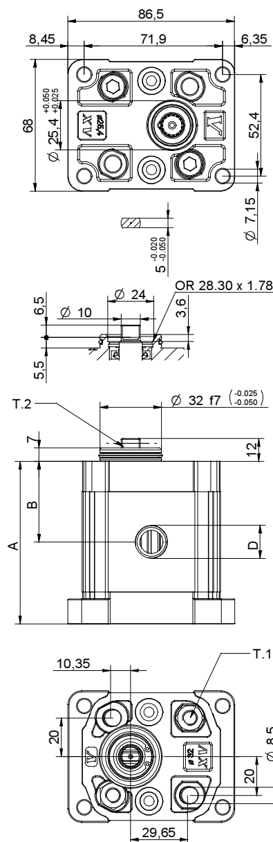
TIPO Peso A B D D kg mm mm IN OUT X1T/0.9 0,950 73,5 36,3 3/8" BSPP 3/8" BSPP X1T/1.2 0,970 74,5 36,8 3/8" BSPP 3/8" BSPP X1T/1.7 1,010 76,0 37,5 3/8" BSPP 3/8" BSPP X1T/2.2 1,030 78,0 38,5 3/8" BSPP 3/8" BSPP X1T/2.6 1,060 80,0 39,5 3/8" BSPP 3/8" BSPP X1T/3.2 1,090 82,0 40,5 3/8" BSPP 3/8" BSPP X1T/3.8 1,120 84,0 41,5 3/8" BSPP 3/8" BSPP X1T/4.3 1,170 86,0 42,5 3/8" BSPP 3/8" BSPP X1T/4.9 1,200 89,0 44,0 3/8" BSPP 3/8" BSPP X1T/5.9 1,260 92,5 45,8 3/8" BSPP 3/8" BSPP X1T/6.5 1,300 95,0 47,0 3/8" BSPP 3/8" BSPP X1T/7.8 1,360 99,0 49,0 3/8" BSPP 3/8" BSPP X1T/9.8 1.500 108,0 53,5 3/8" BSPP 3/8" BSPP
